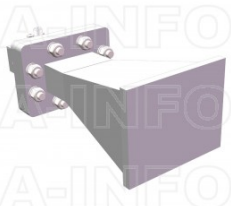
LB-137-10-C-SFSPO Standard Gain Horn Antenna 5.85-8.2GHz 10dB Gain SMA Female
